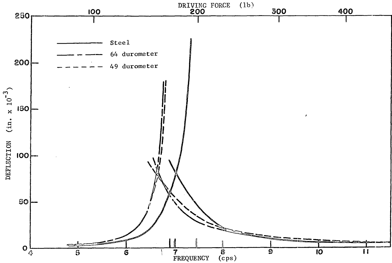
Fig. 60. Deflection-frequency curves for beam 3-1, oscillator with concrete blocks, W = 3.48 lb, e = 4.51 in.
