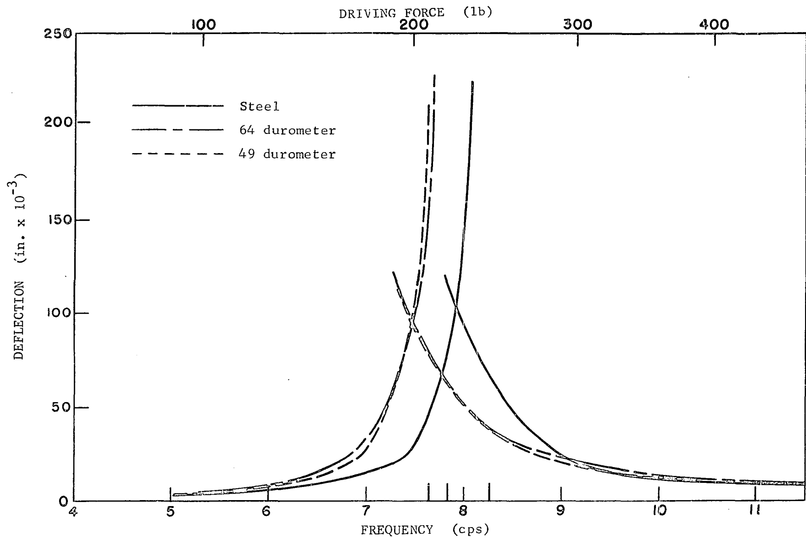
Fig. 48. Deflection-frequency curves for beam 3-1, oscillator only, W = 3.48 lb, e = 4.51 in.
