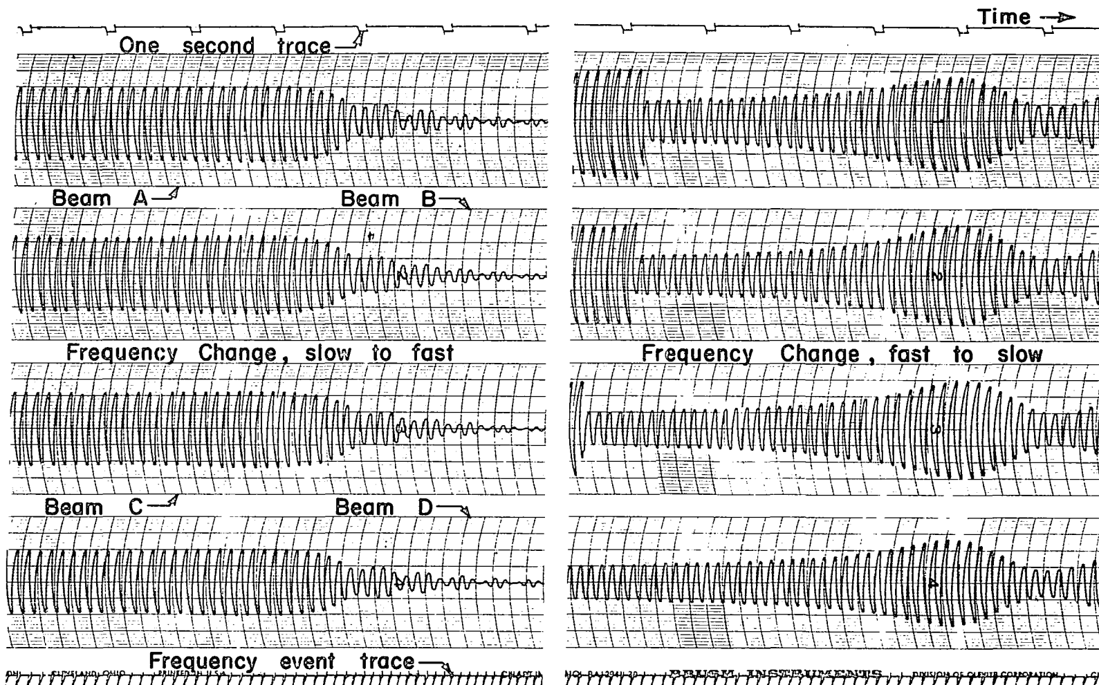
Fig. 15. Typical oscillograph chart--strain
