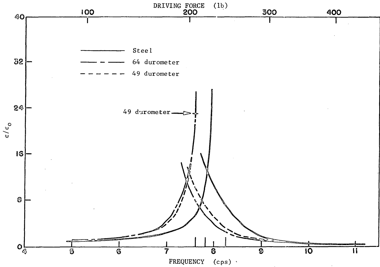
Fig. 34. Strain amplification factor-frequency curves for beam C, oscillator only, W = 3.48 lb, e = 4.51 in.
