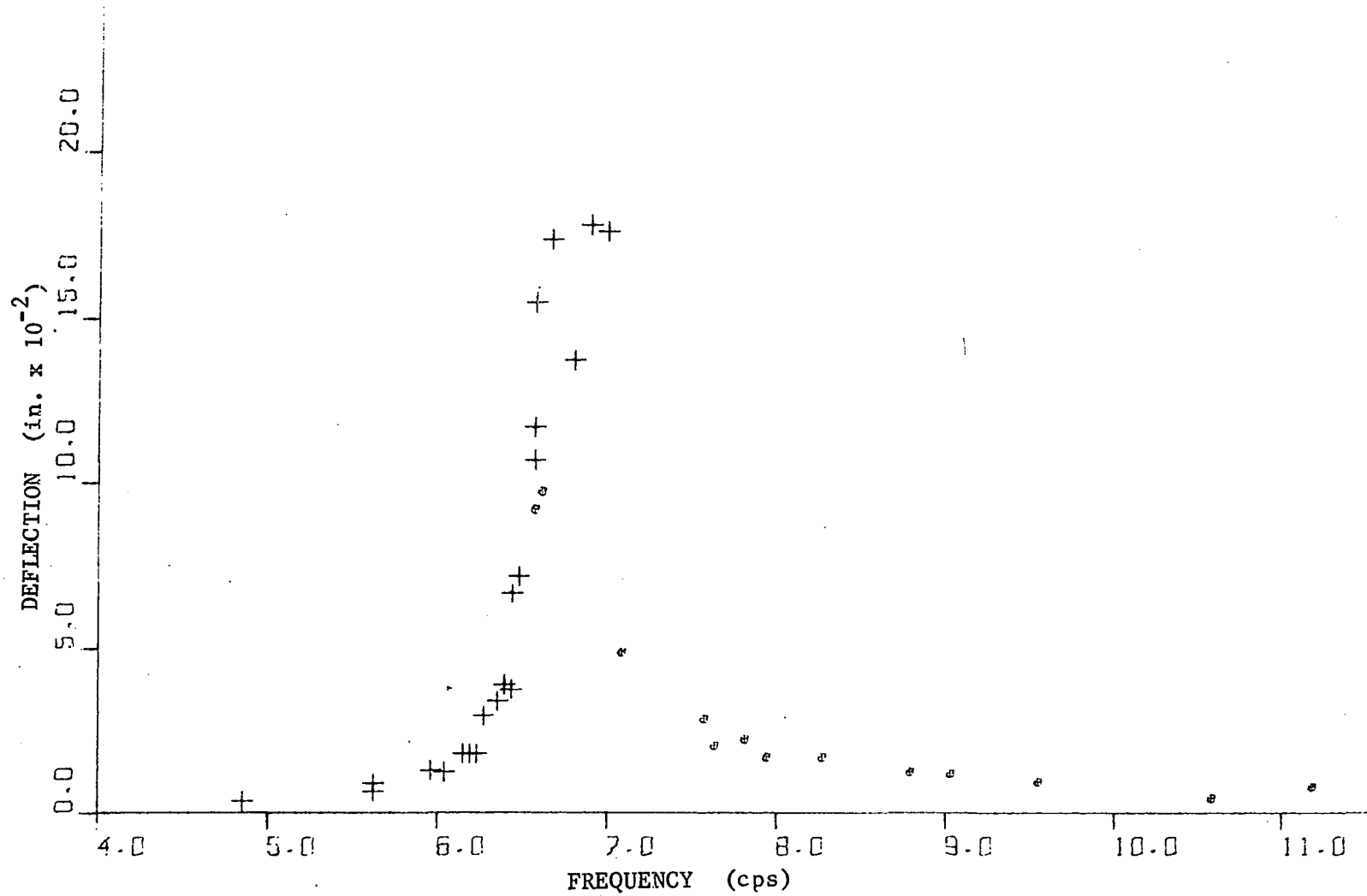
Fig. 26. Computer plot of deflection-frequency relationship for beam 3-1, 64 durometer neoprene pads, oscillator with concrete blocks, W = 3.48 lb, e = 4.51 in.
