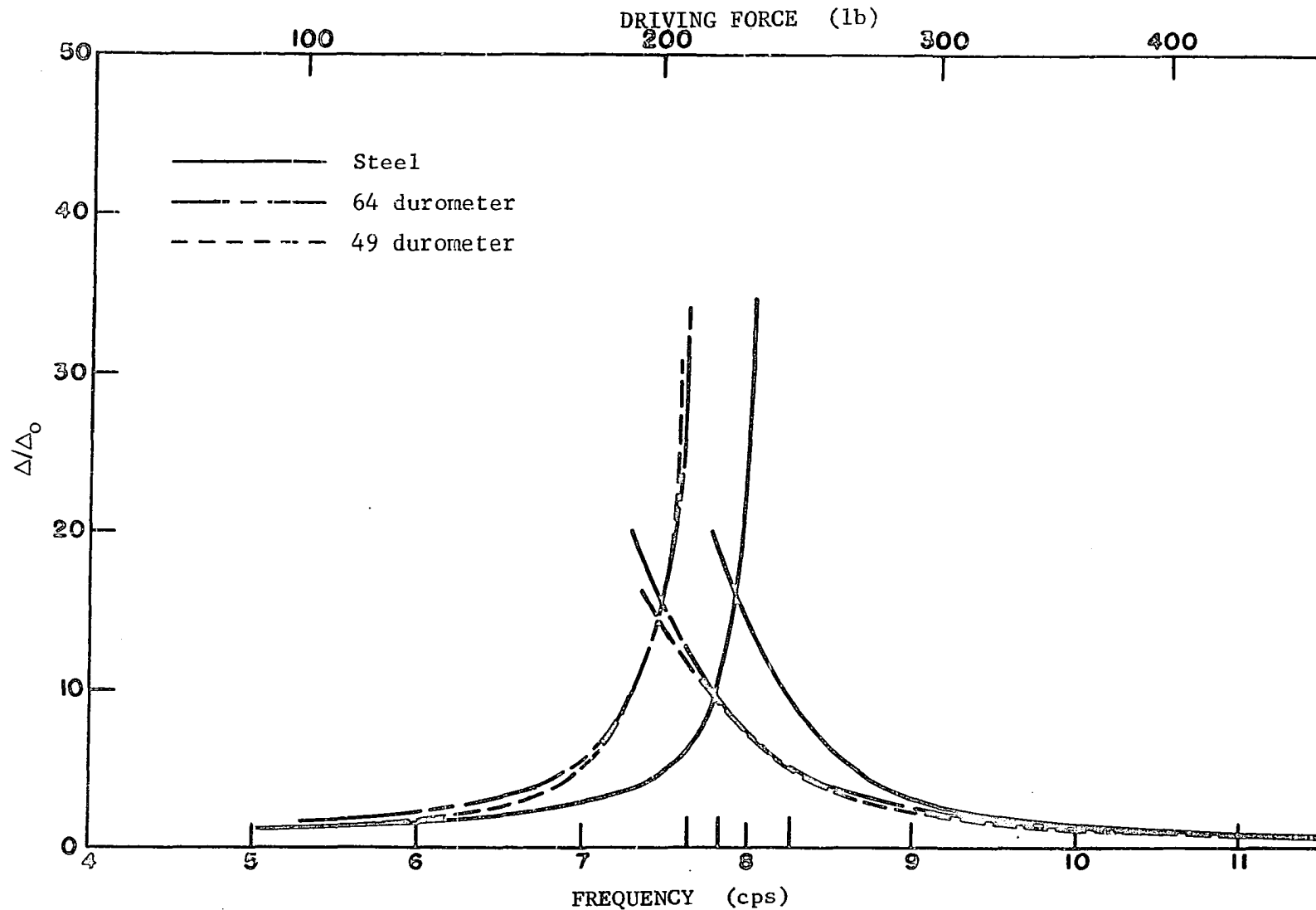
Fig. 50. Deflection amplification factor-frequency curves for beam 3-1, oscillator only, W = 3.48 lb, e = 4.51 in.
