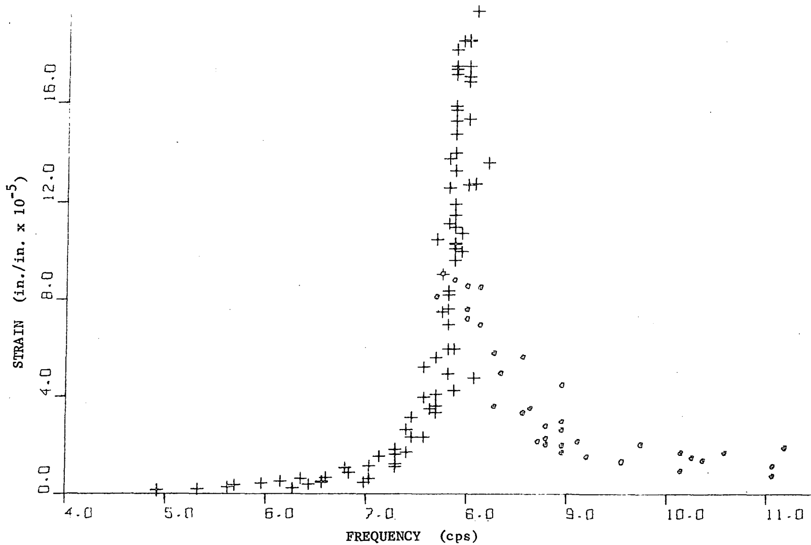
Fig. 23. Computer plot of strain-frequency relationship for beam A, curved steel sole plates, oscillator only, W = 3.48 lb, e = 4.51 in.
