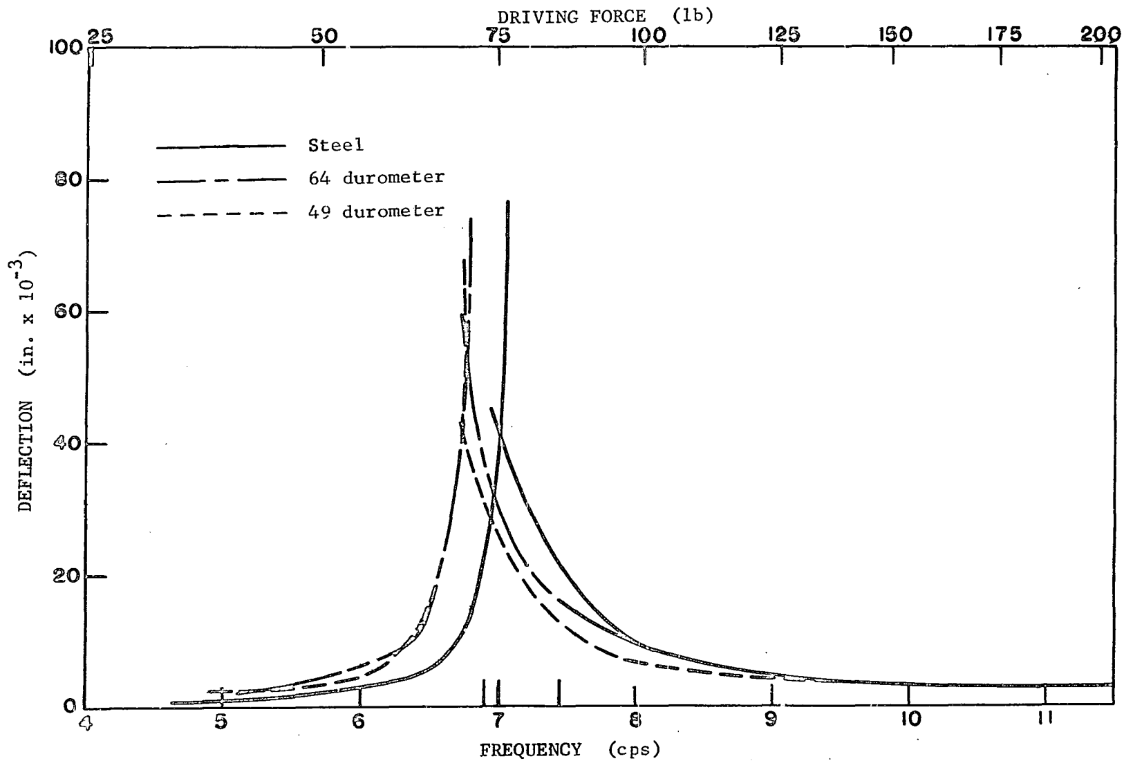
Fig. 58. Deflection-frequency curves for beam 3-1, oscillator with concrete blocks, W = 0.82 lb, e = 7.01 in.
