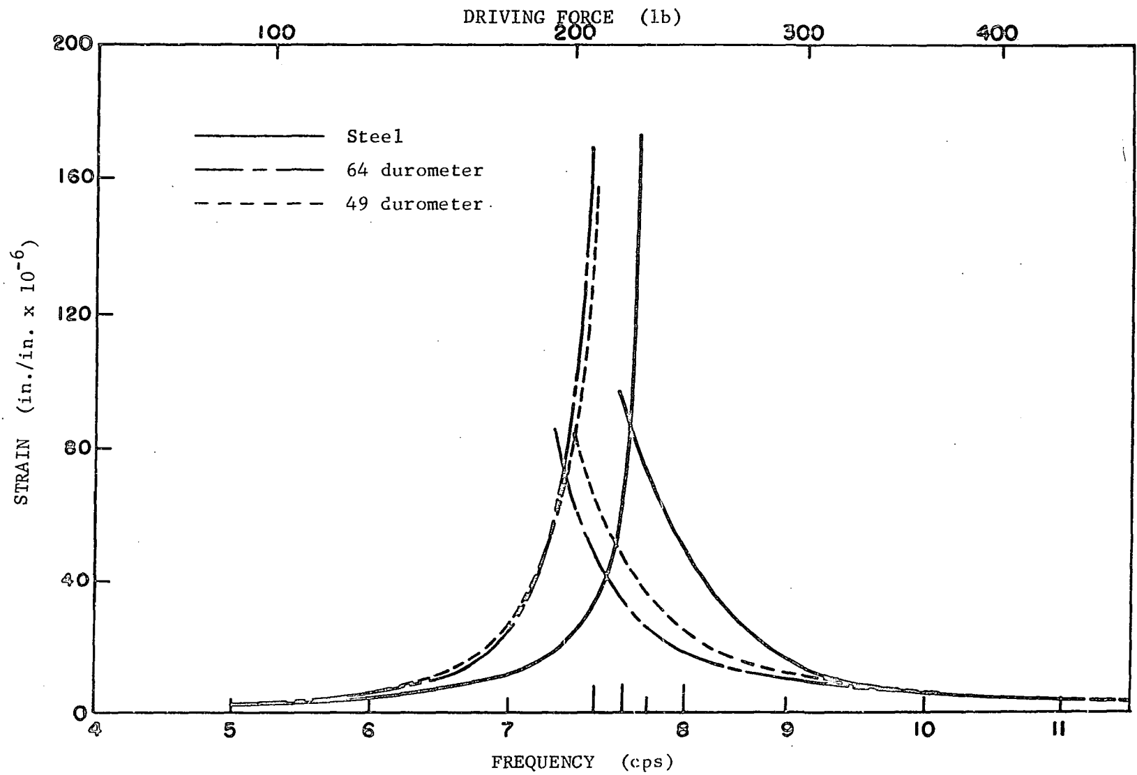
Fig. 30. Strain-frequency curves for beam C, oscillator only, W = 3.48 lb, e = 4.51 in.
