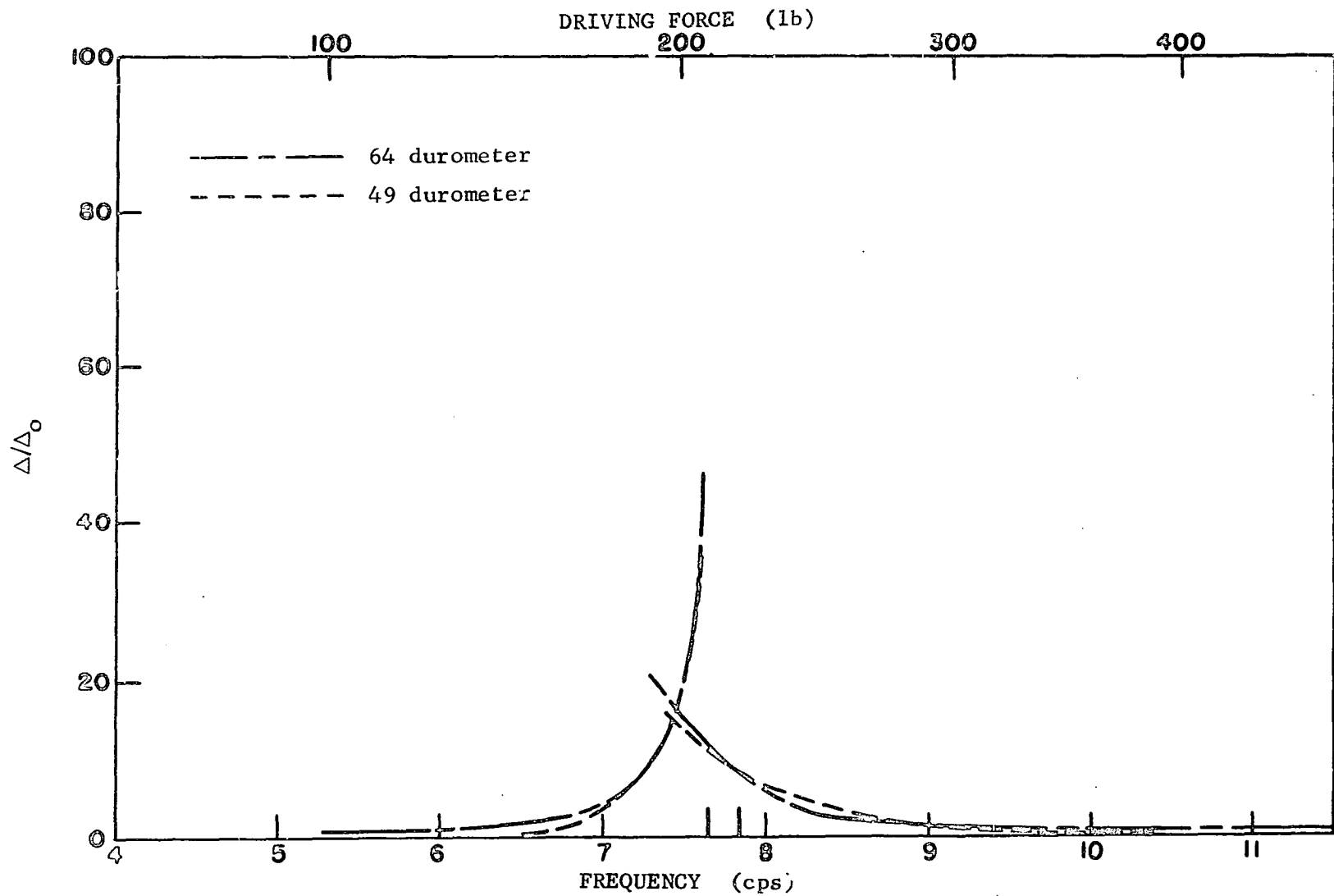
Fig. 52. Deflection amplification factor-frequency curves for north end of beam 3-1, oscillator only, W = 3.48 lb, e = 4.51 in.
