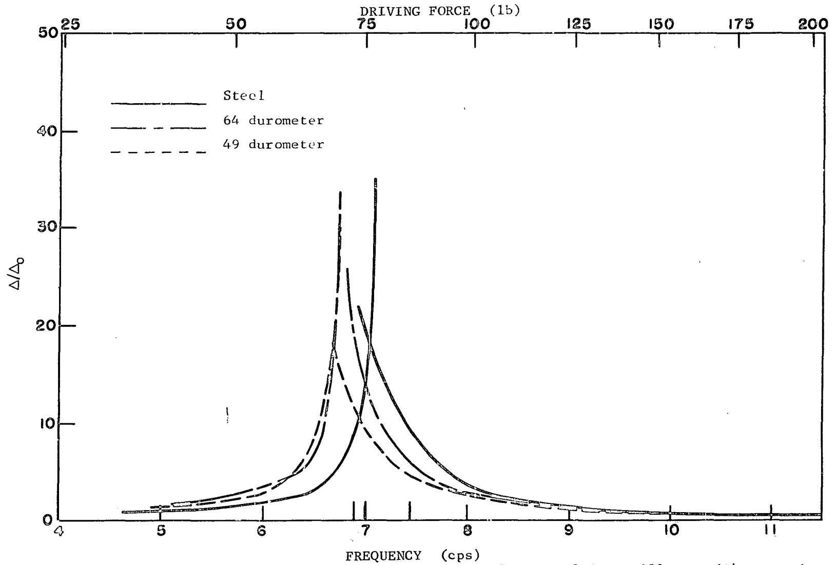
Fig. 63. Deflection amplification factor-frequency curves for beam 3-1, oscillator with concrete blocks, W = 0.82 lb, e = 7.01 in.
