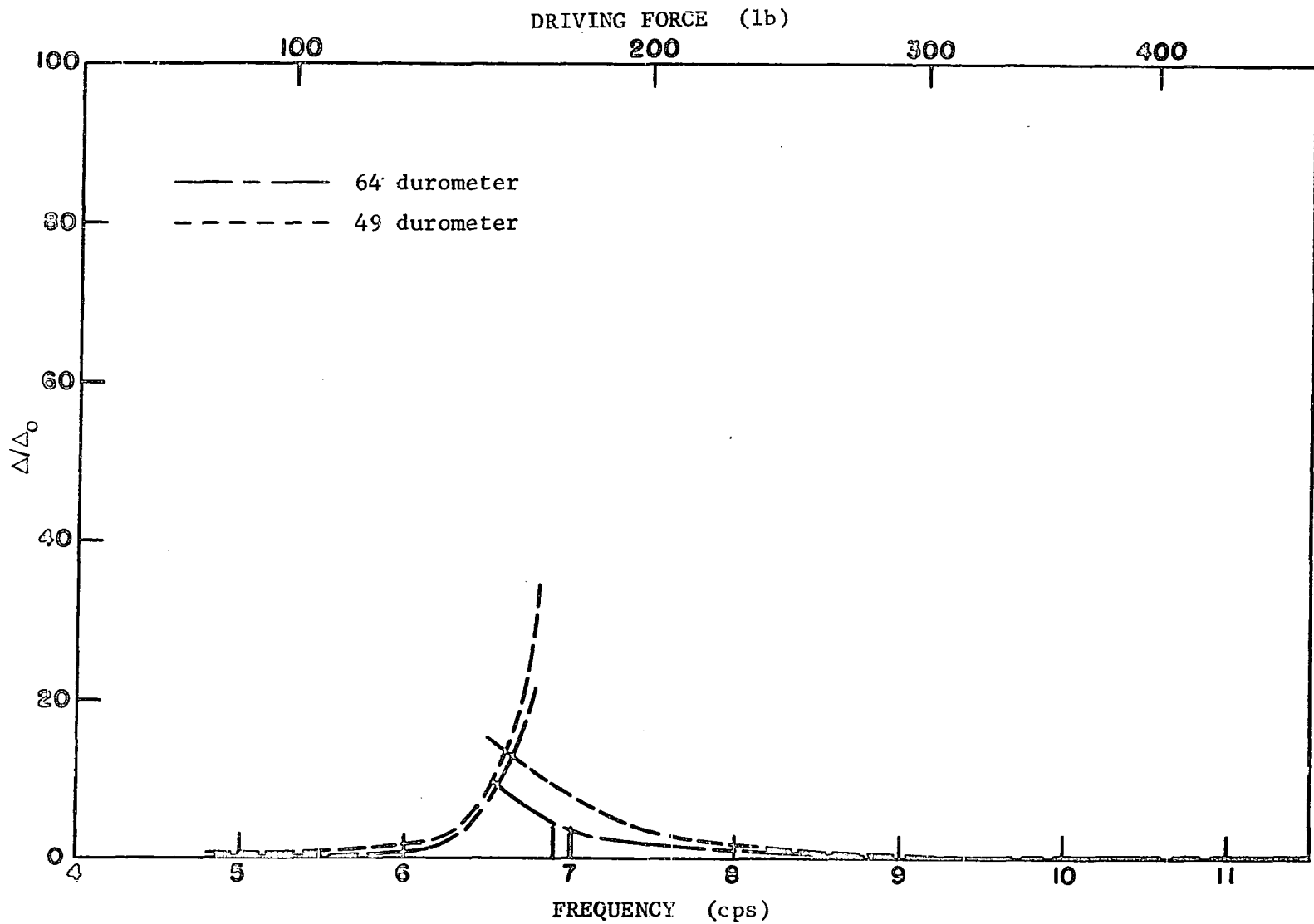
Fig. 68. Deflection amplification factor-frequency curves for north end of beam 3-1, oscillator with concrete blocks, W = 3.48 lb, e = 4.51 in.
