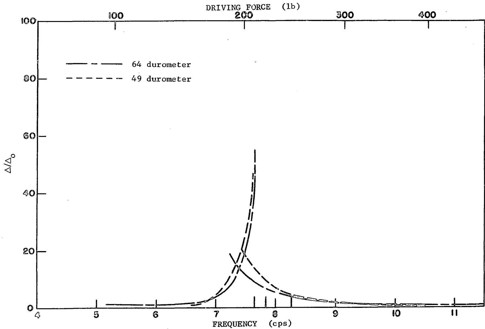
Fig. 54. Deflection amplification factor-frequency curves for south end of beam 3-1, oscillator only, W = 3.48 lb, e = 4.51 in.
