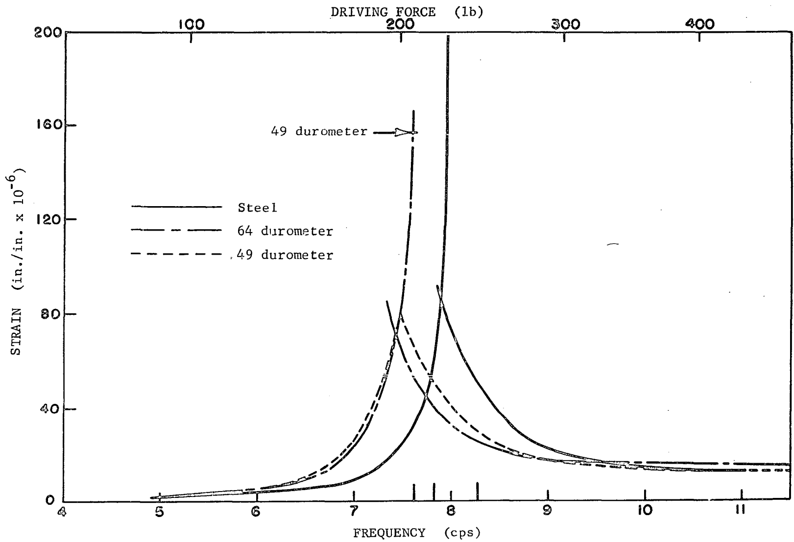
Fig. 29. Strain-frequency curves for beam A, oscillator only, W = 3.48 lb, e = 4.51 in.
