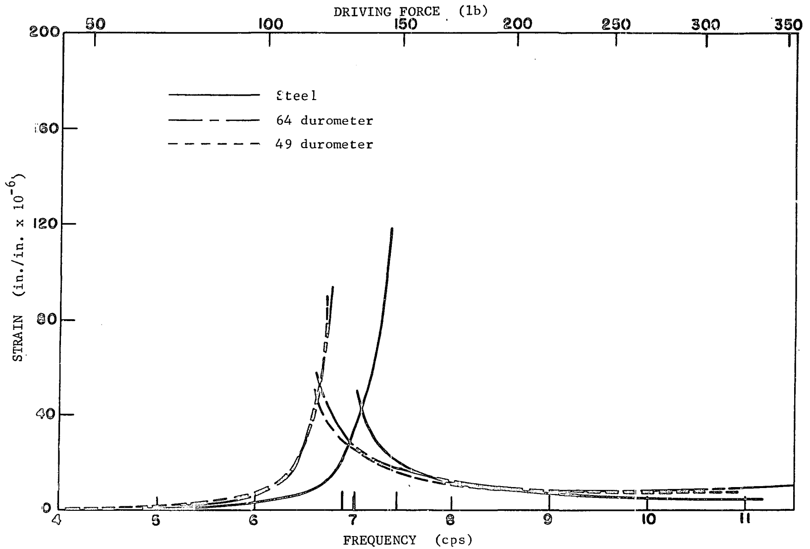
Fig. 38. Strain-frequency curves for beam A, oscillator with concrete blocks, W = 3.48 lb, e = 3.26 in.
