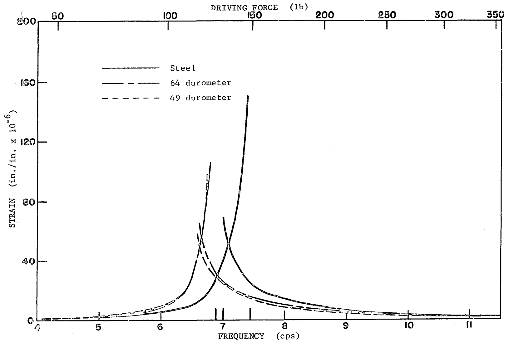
Fig. 41. Strain-frequency curves for beam C, oscillator with concrete blocks, W = 3.48 lb, e = 3.26 in.
