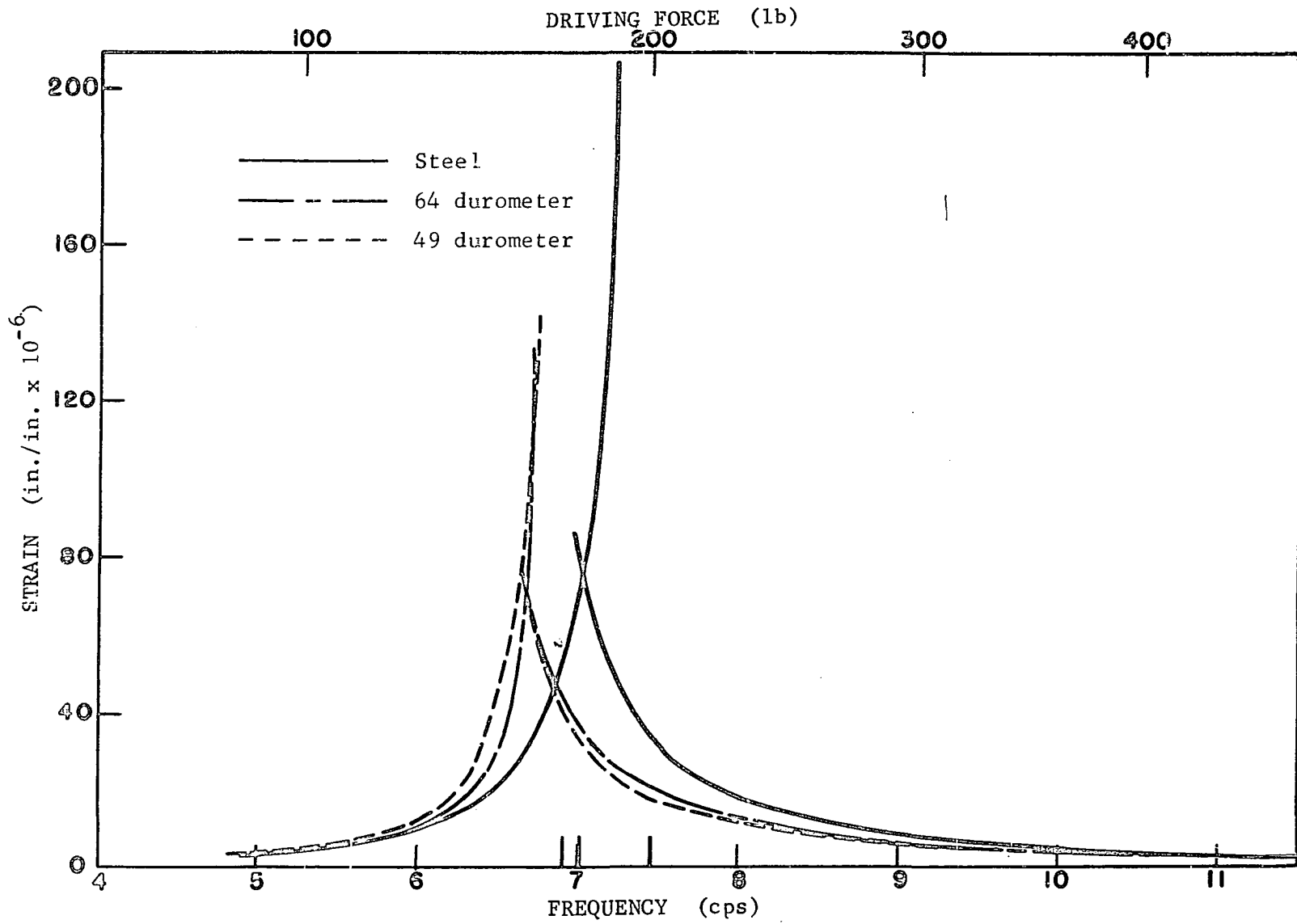
Fig. 42. Strain-frequency curves for beam C, oscillator with concrete blocks, W = 3.48 lb, e = 4.51 in.
