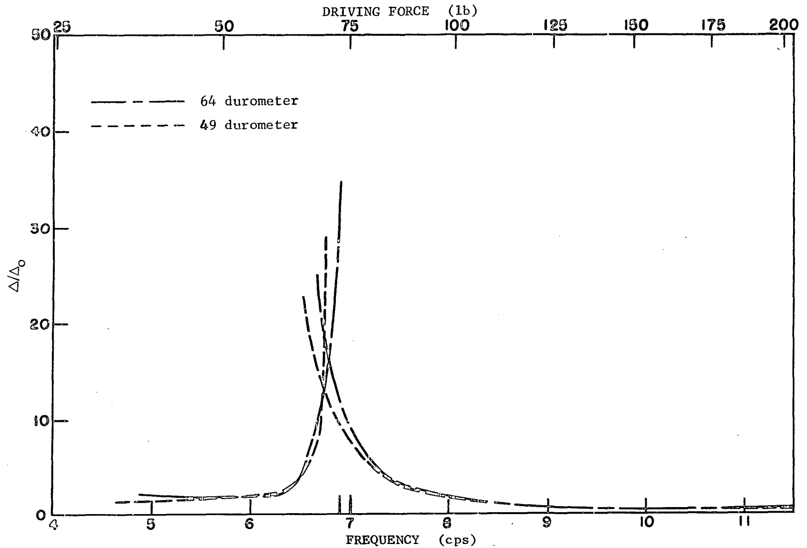
Fig. 65. Deflection amplification factor-frequency curves for north end of beam 1-1, oscillator with concrete blocks, W = 0.82 lb, e = 7.01 in.
