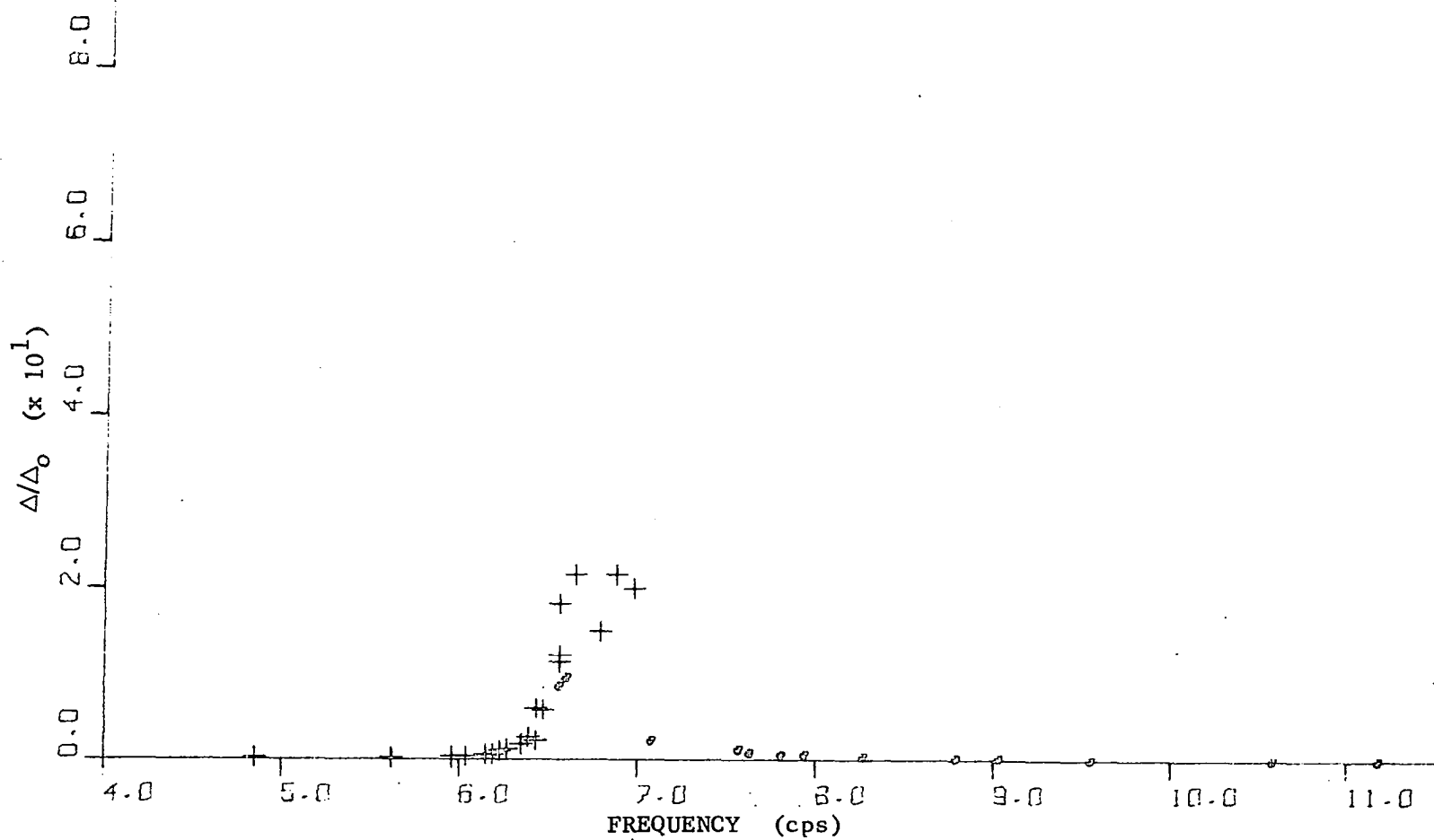
Fig. 28. Computer plot of deflection amplification factor-frequency relationship for north end of beam 3-1, 64 durometer neoprene pads, oscillator with concrete blocks, W = 3.48 lb, e = 4.51 in.
