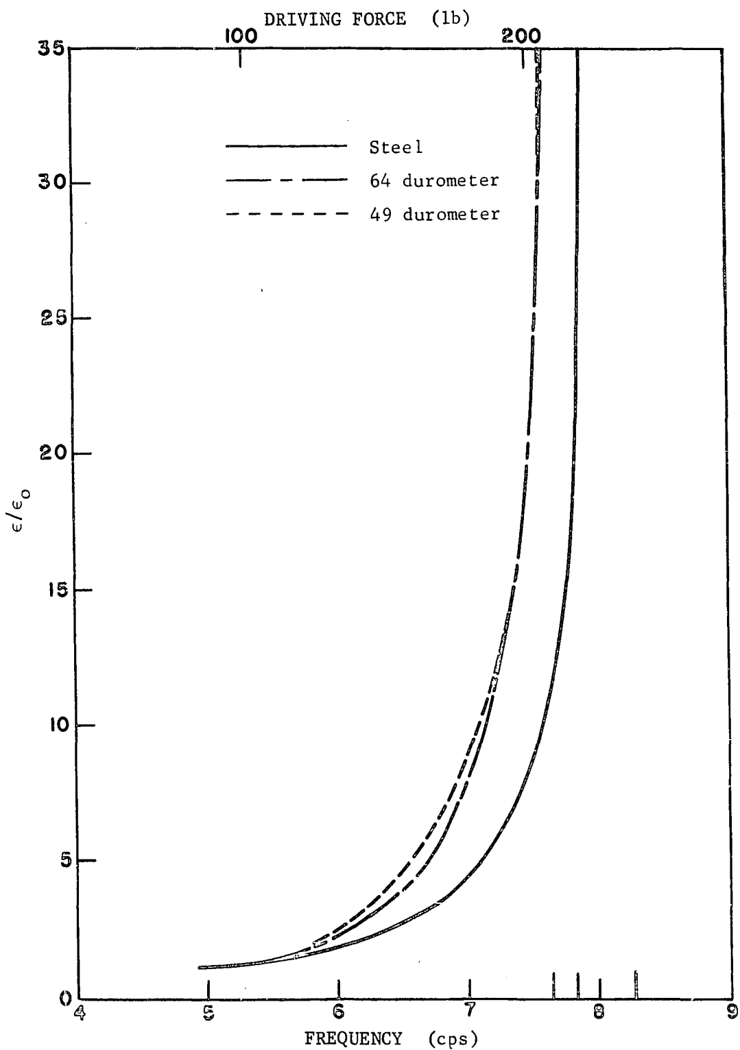
Fig. 35. Partial strain amplification factor-frequency curves for beam A, oscillator only, W = 3.48 lb, e = 4.51 in.
