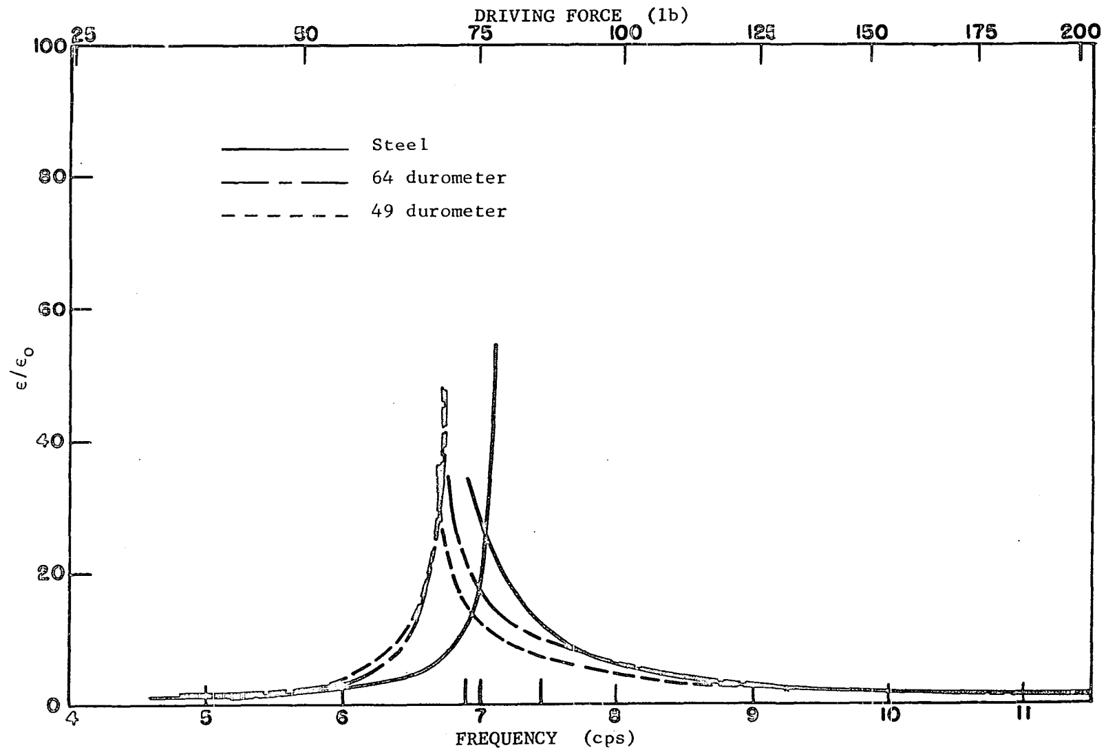
Fig. 43. Strain amplification factor-frequency curves for beam A, oscillator with concrete blocks, W = 0.82 lb, e = 7.01 in.
