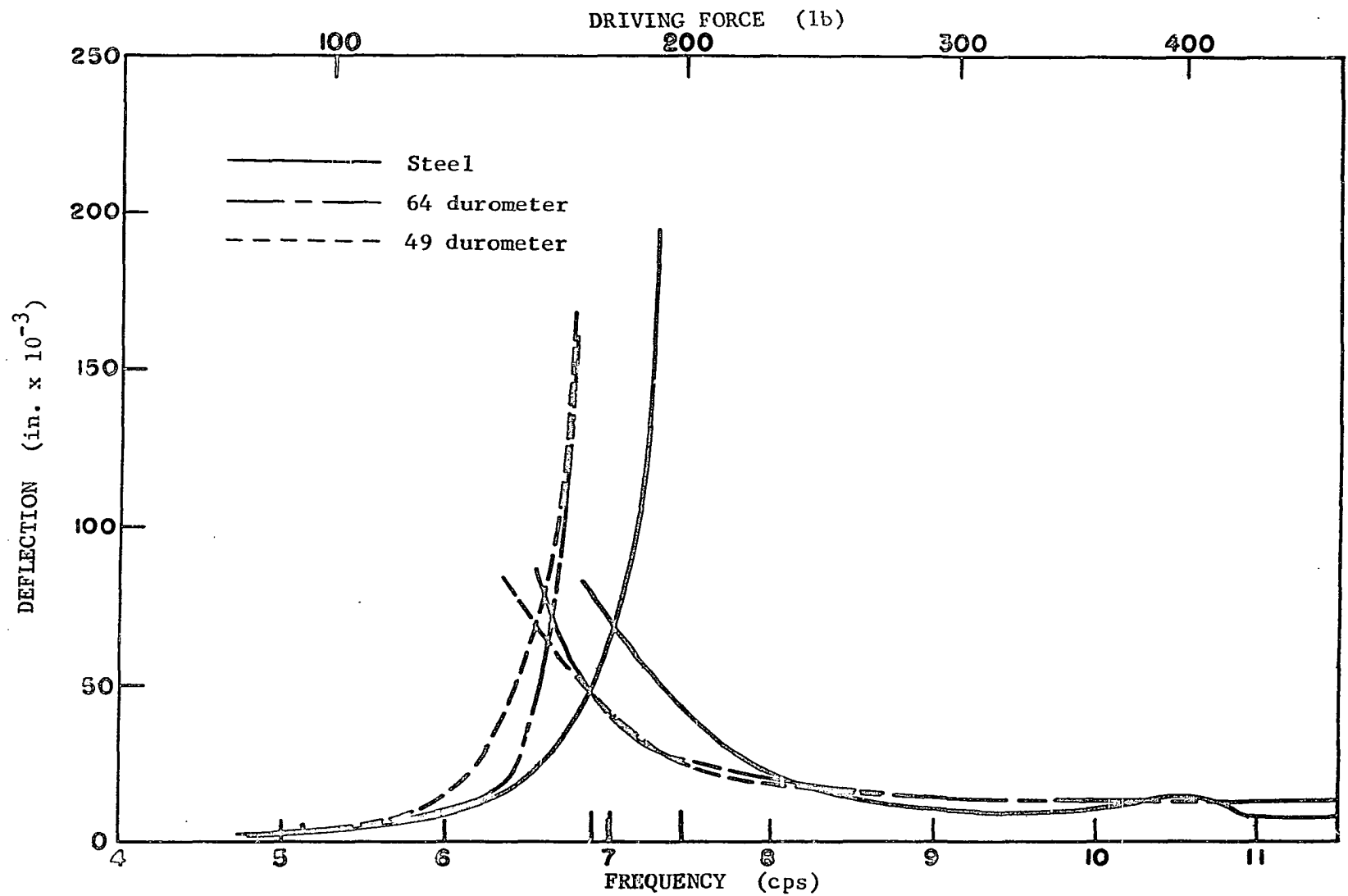
Fig. 57. Deflection-frequency curves for beam 1-1, oscillator with concrete blocks, W = 3.48 lb, e = 4.51 in.
