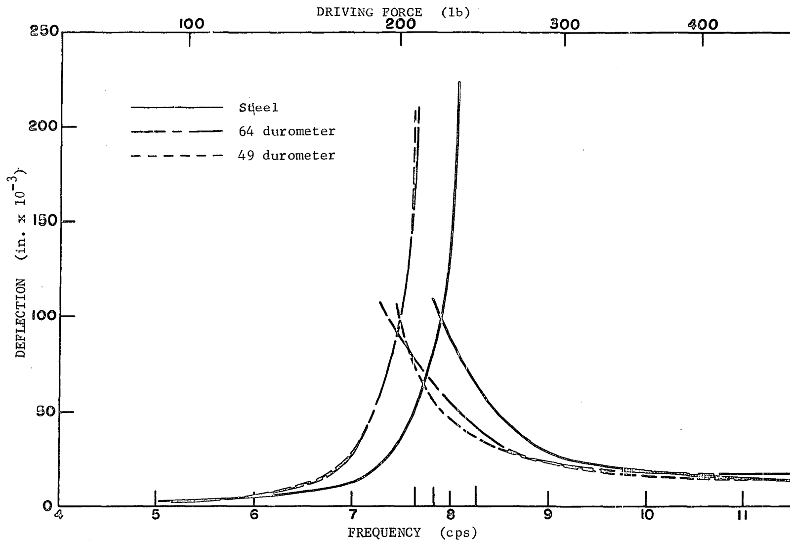
Fig. 47. Deflection-frequency curves for beam 1-1, oscillator only, W = 3.48 lb, e = 4.51 in.
