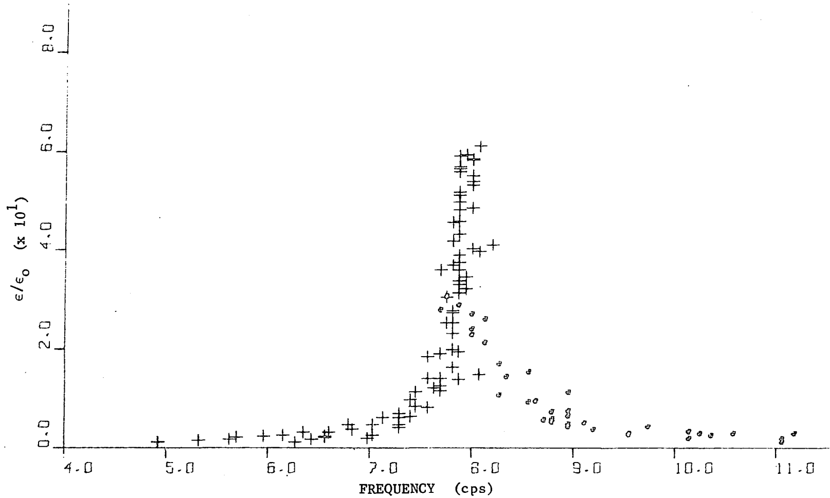
Fig. 25. Computer plot of strain amplification factor-frequency relationship for beam A, curved steel sole plates, oscillator only, W = 3.48 \text{ lb} , e = 4.51 \text{ in} .
