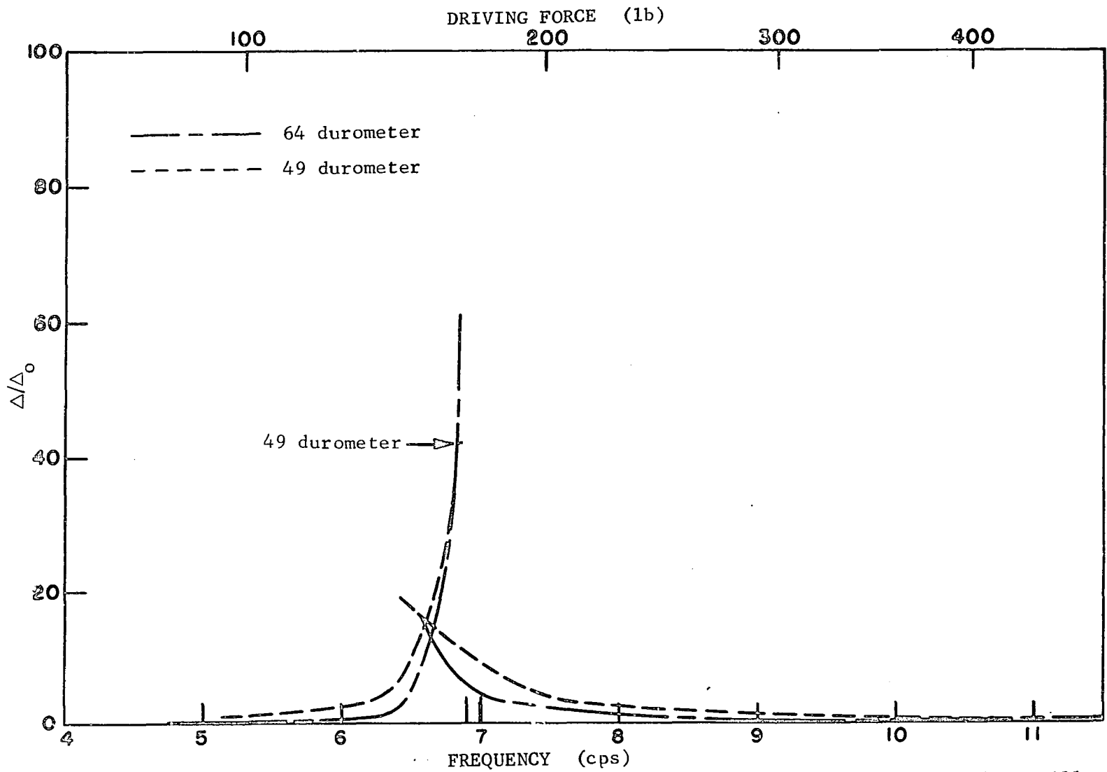
Fig. 69. Deflection amplification factor-frequency curves for south end of beam 1-1, oscillator with concrete blocks, W = 3.48 lb, e = 4.51 in.
