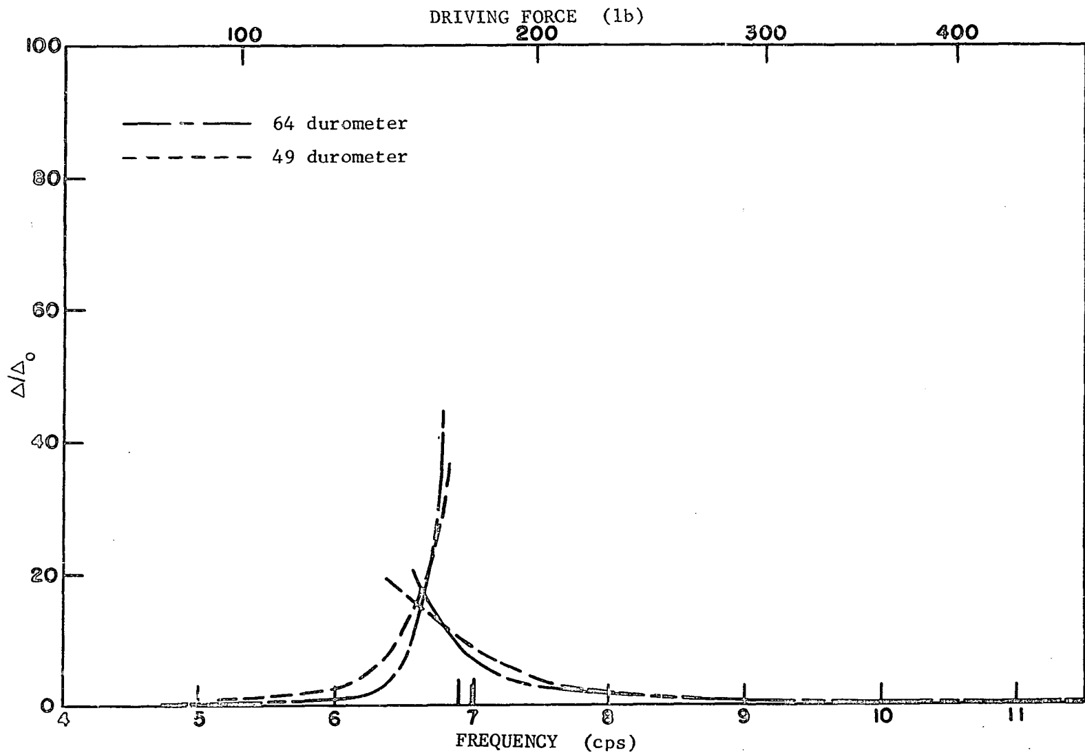
Fig. 66. Deflection amplification factor-frequency curves for north end of beam 1-1, oscillator with concrete blocks, W = 3.48 lb, e = 4.51 in.
