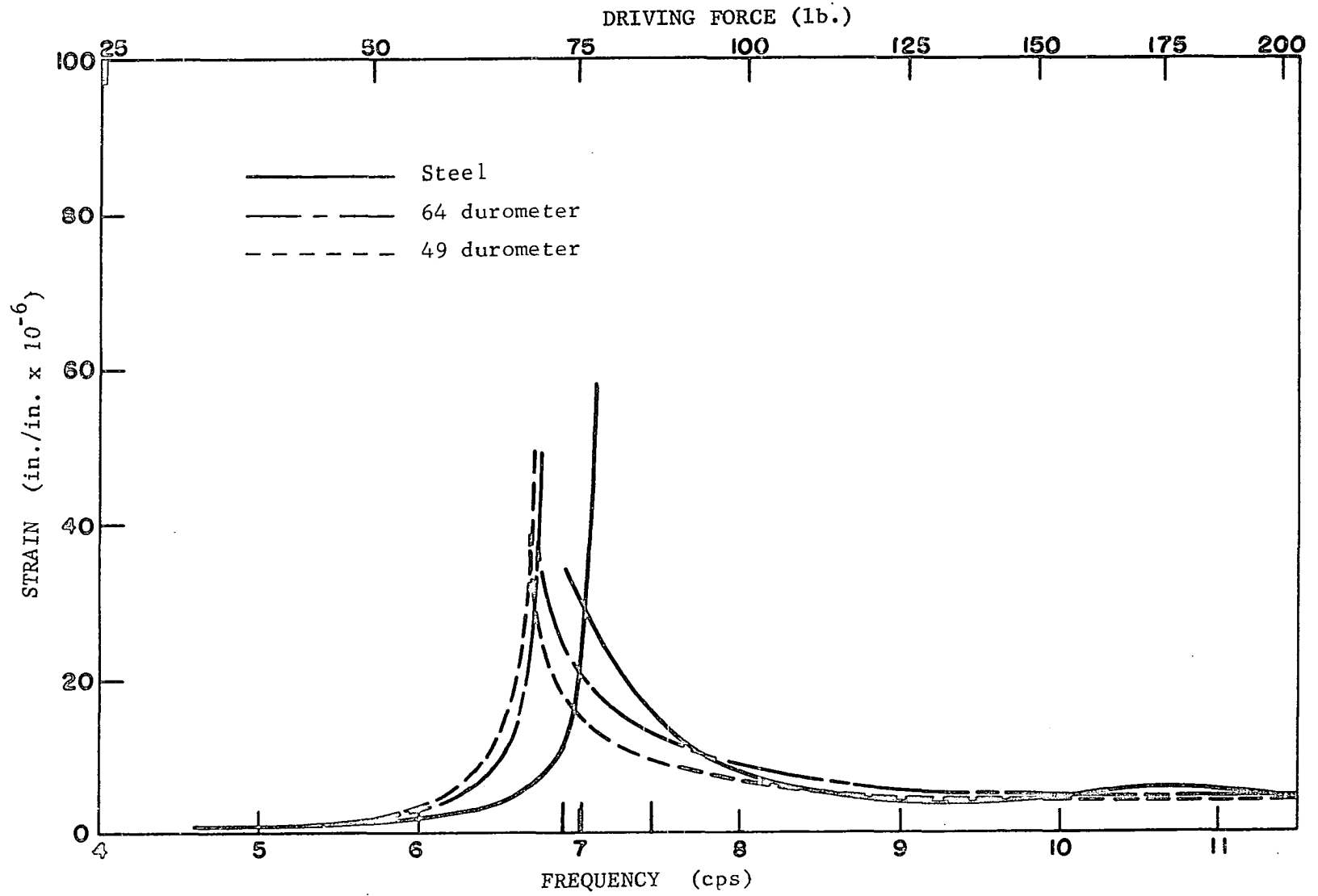
Fig. 37. Strain-frequency curves for beam A, oscillator with concrete blocks, W = 0.82 lb, e = 7.01 in.
