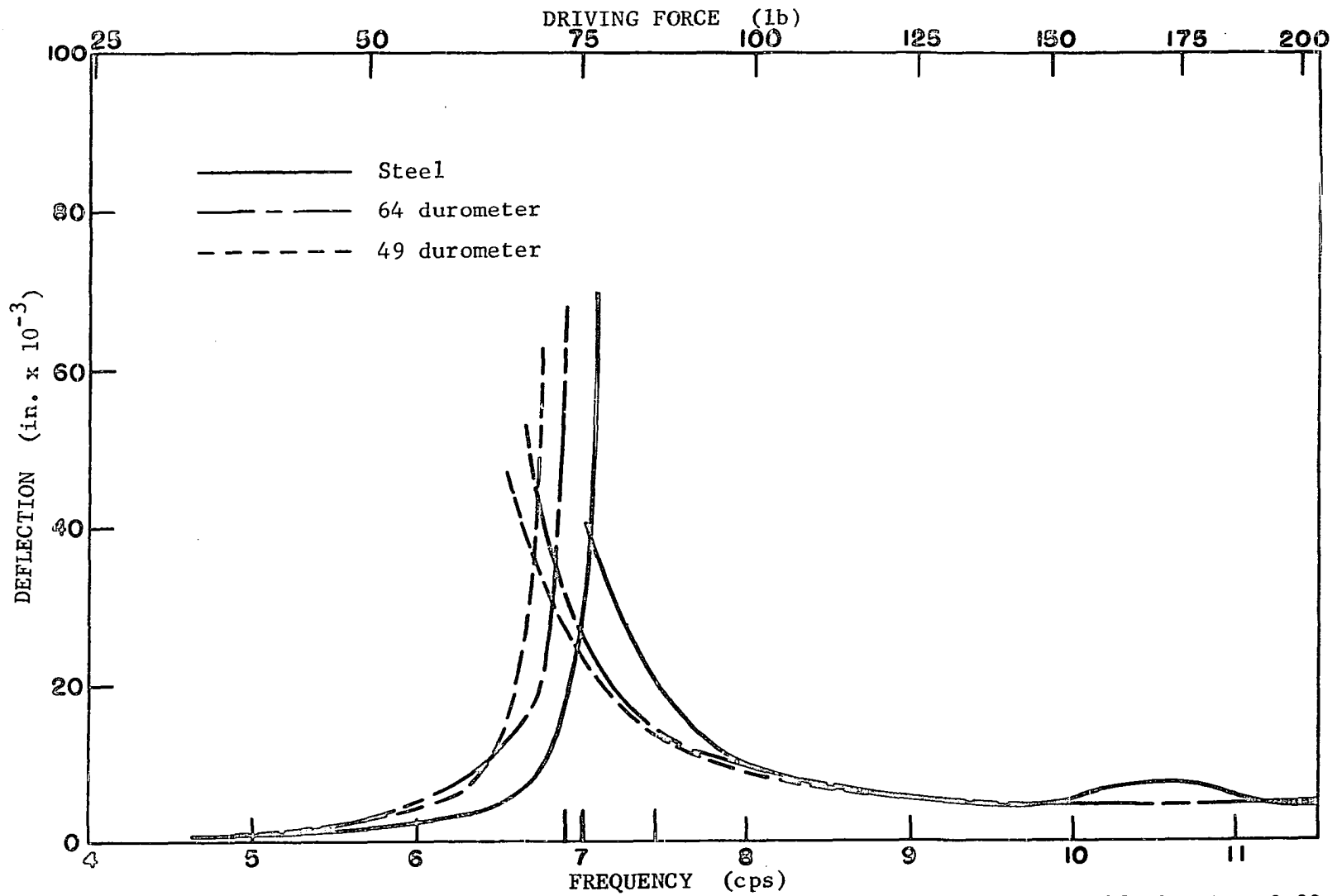
Fig. 55. Deflection-frequency curves for beam 1-1, oscillator with concrete blocks, W = 0.82 lb, e = 7.01 in.
