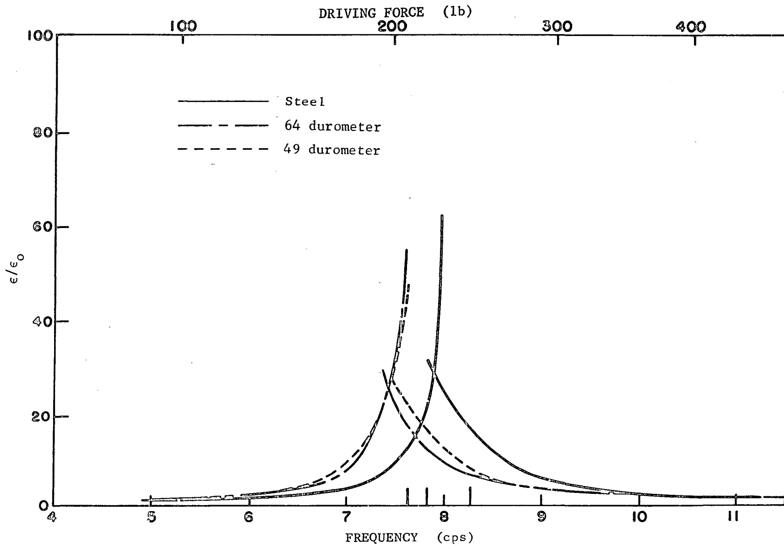
Fig. 33. Strain amplification factor-frequency curves for beam A, oscillator only, W = 3.48 lb, e = 4.51 in.
