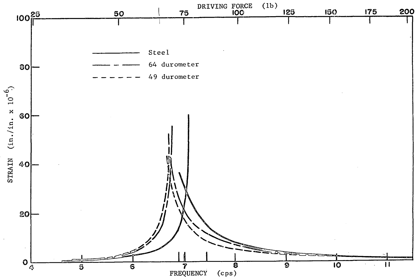
Fig. 40. Strain-frequency curves for beam C, oscillator with concrete blocks, W = 0.82 lb, e = 7.01 in.
