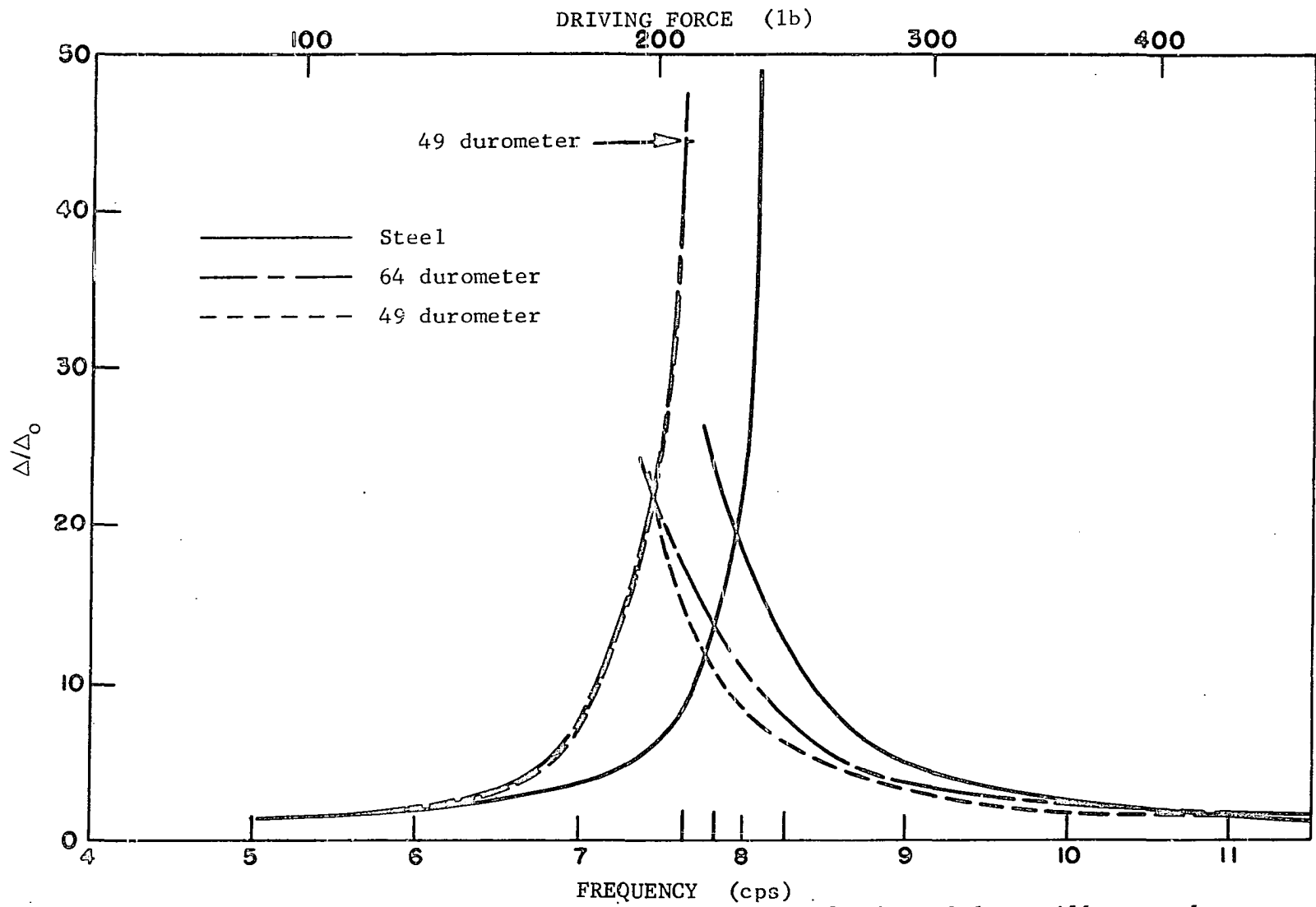
Fig. 49. Deflection amplification factor-frequency curves for beam 1-1, oscillator only, W = 3.48 lb, e = 4.51 in.
