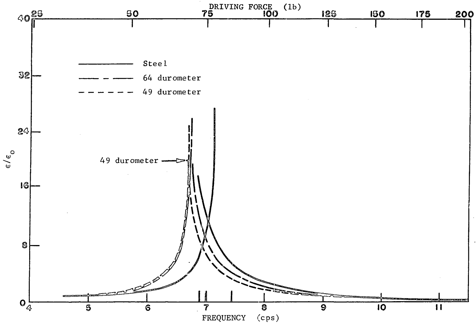
Fig. 45. Strain amplification factor-frequency curves for beam C, oscillator with concrete blocks, W = 0.82 lb, e = 7.01 in.
