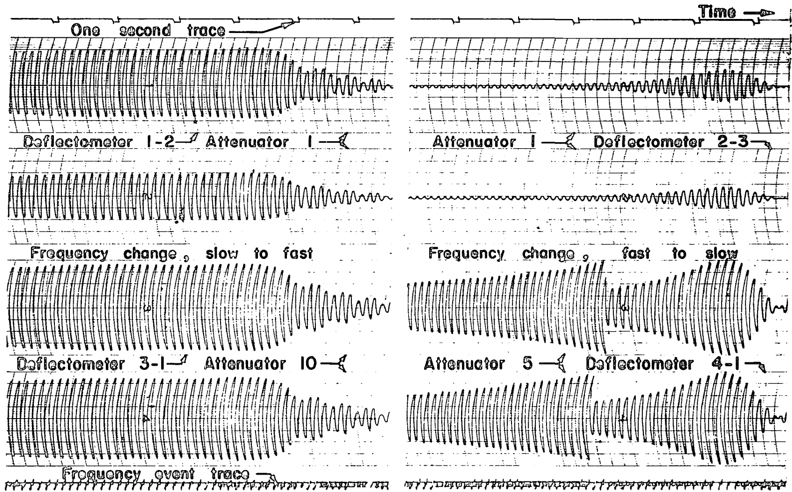
Fig. 16. Typical oscillograph chart--deflection
