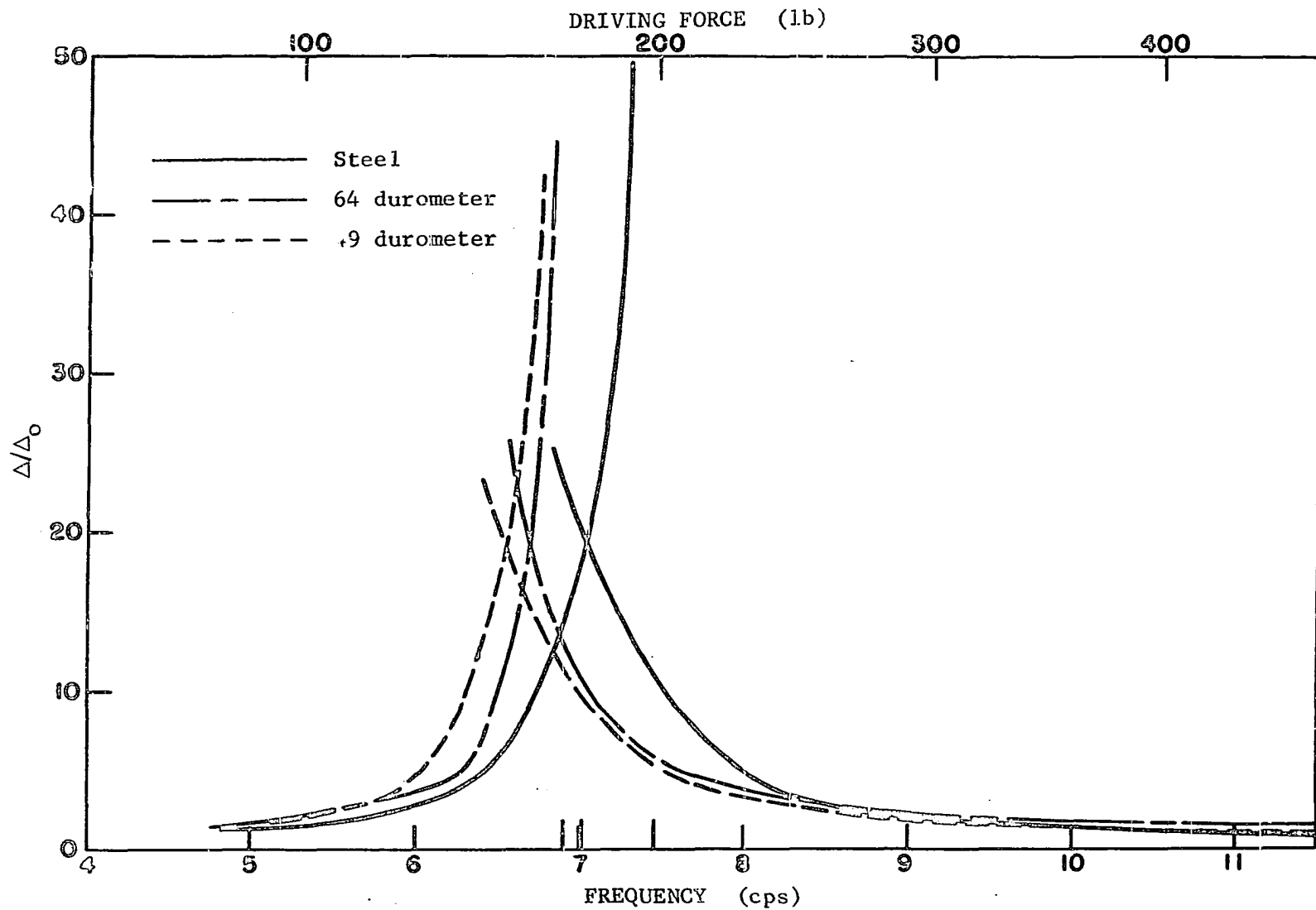
Fig. 62. Deflection amplification factor-frequency curves for beam 1-1, oscillator with concrete blocks, W = 3.48 lb, e = 4.51 in.
