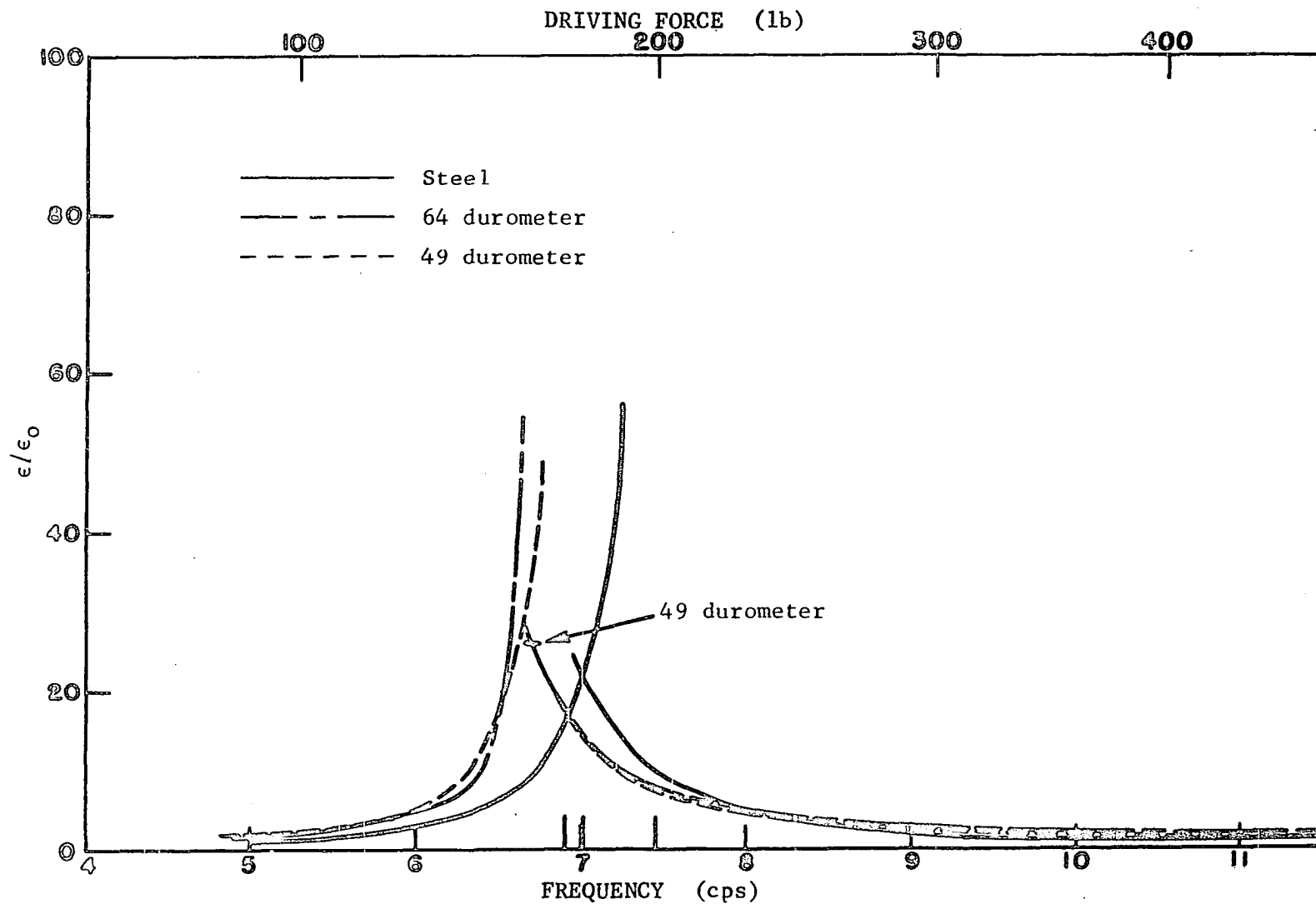
Fig. 44. Strain amplification factor-frequency curves for beam A, oscillator with concrete blocks, W = 3.48 lb, e = 4.51 in.
