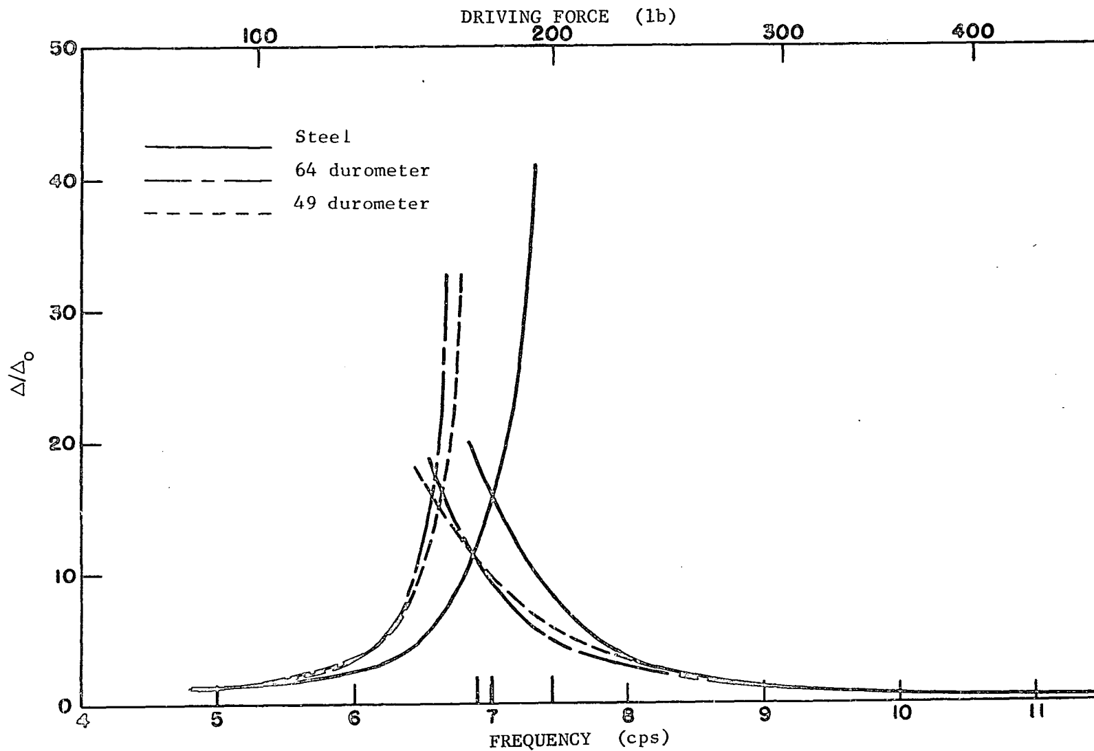
Fig. 64. Deflection amplification factor-frequency curves for beam 3-1, oscillator with concrete blocks, W = 3.48 lb, e = 4.51 in.
