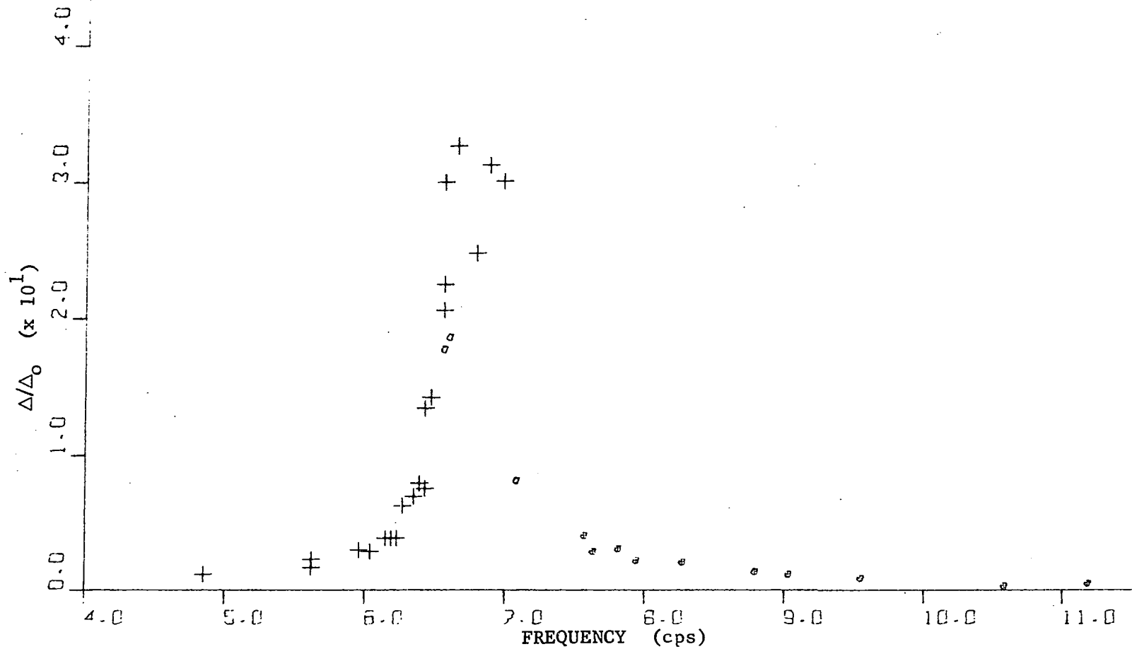
Fig. 27. Computer plot of deflection amplification factor-frequency relationship for beam 3-1, 64 durometer neoprene pads, oscillator with concrete blocks, W = 3.48 lb, e = 4.51 in.
