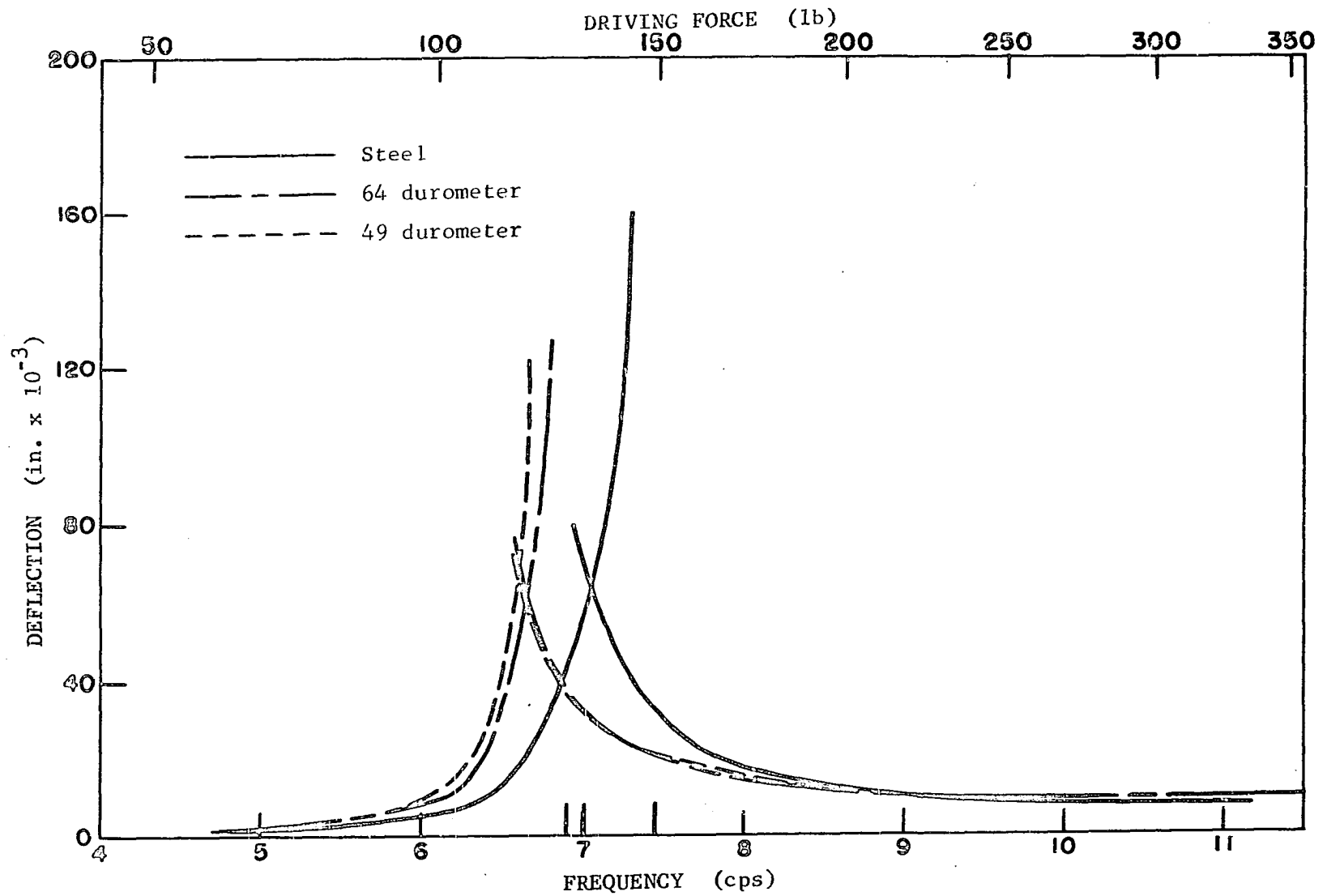
Fig. 56. Deflection-frequency curves for beam 1-1, oscillator with concrete blocks, W = 3.48 lb, e = 3.26 in.
