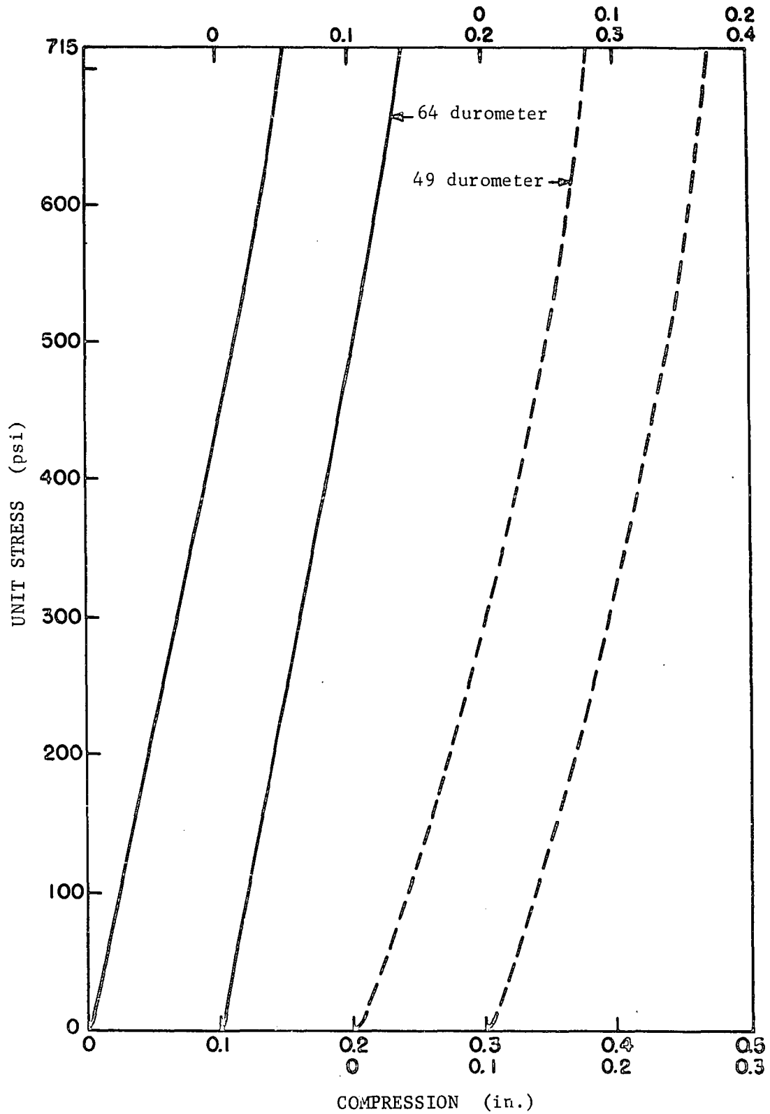
Fig. 12. Stress-deflection curves for neoprene pads
