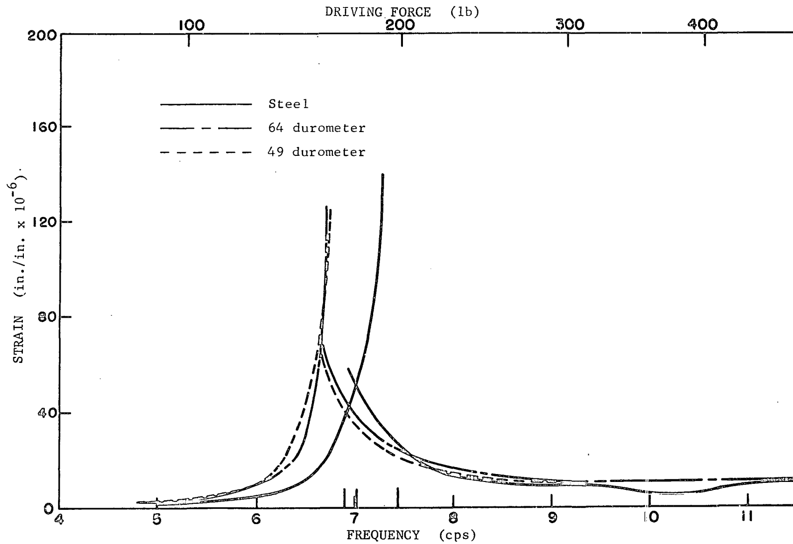
Fig. 39. Strain-frequency curves for beam A, oscillator with concrete blocks, W = 3.48 lb, e = 4.51 in.
