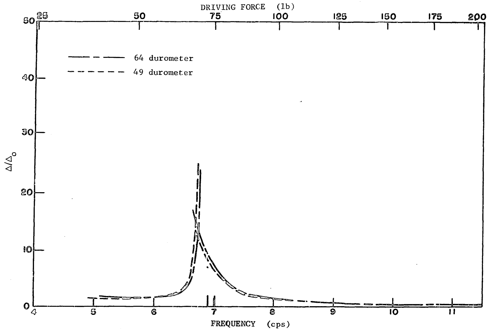
Fig. 67. Deflection amplification factor-frequency curves for north end of beam 3-1, oscillator with concrete blocks, W = 0.82 lb, e = 7.01 in.
