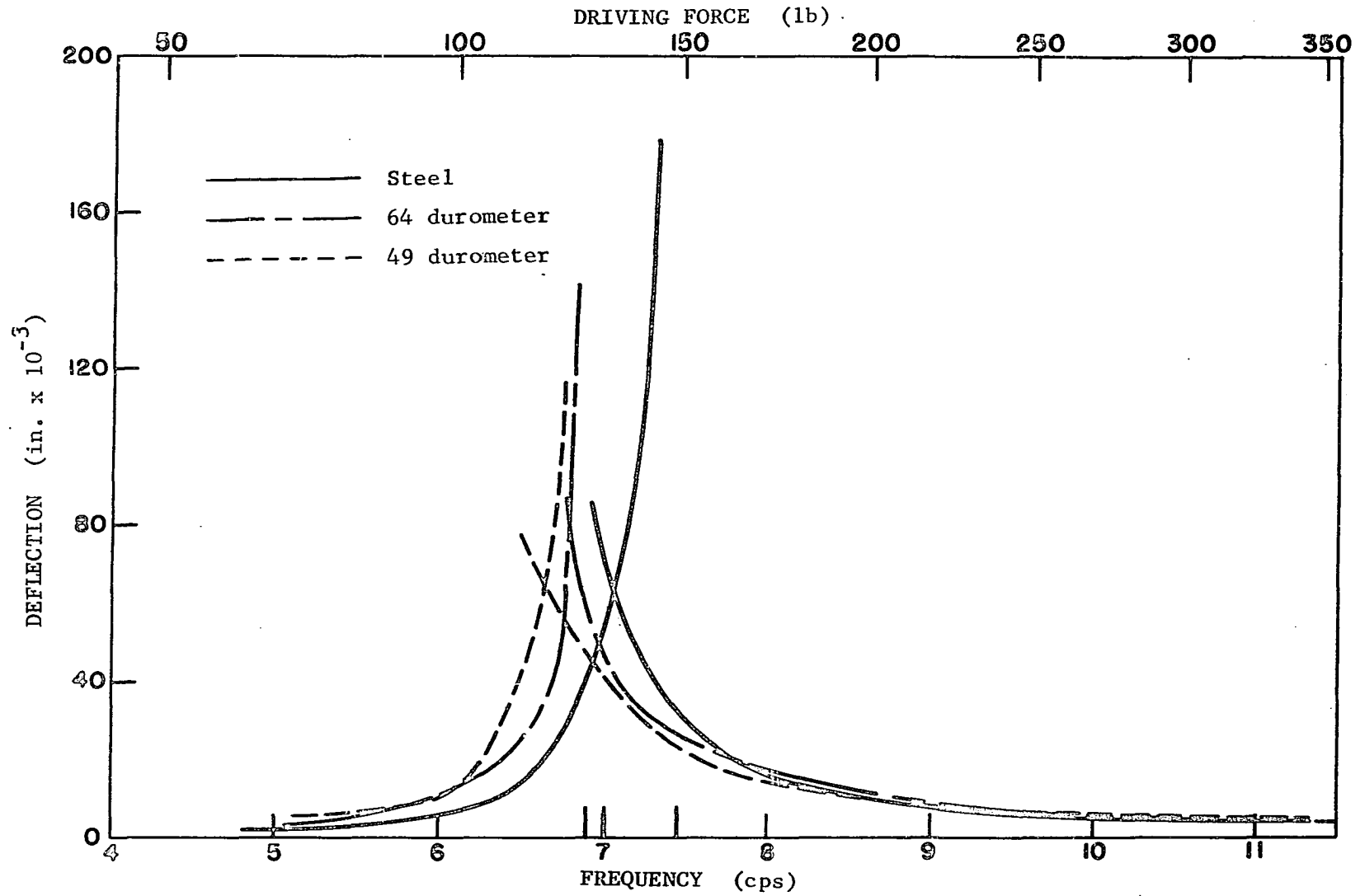
Fig. 59. Deflection-frequency curves for beam 3-1, oscillator with concrete blocks, W = 3.48 lb, e = 3.26 in.
